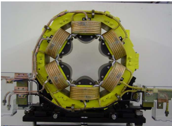
Sextupole magnet
