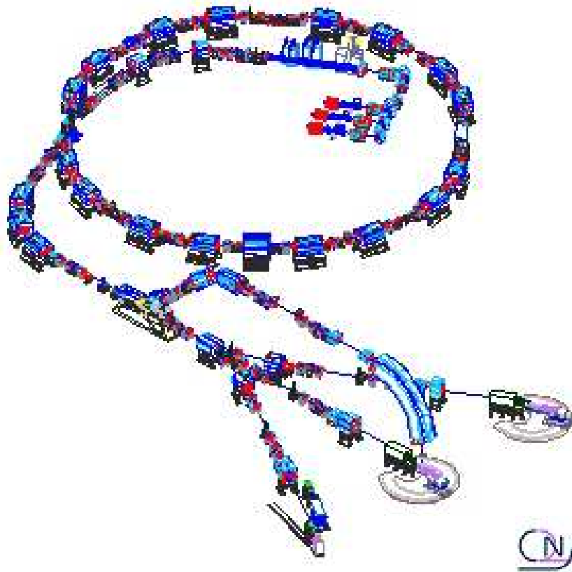
CNAO Synchrotron system
