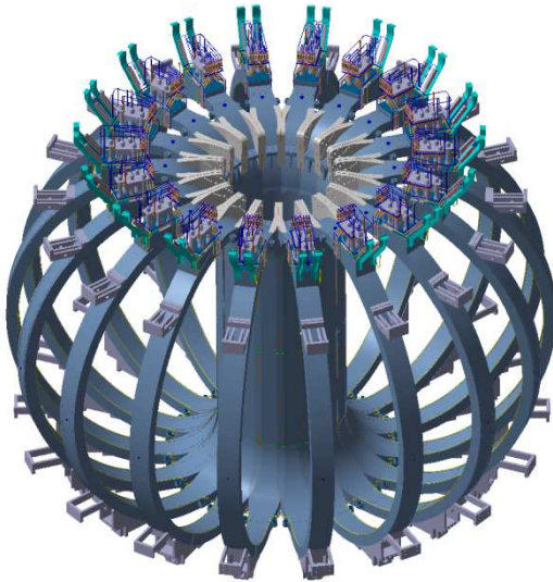
TF coils assembly
